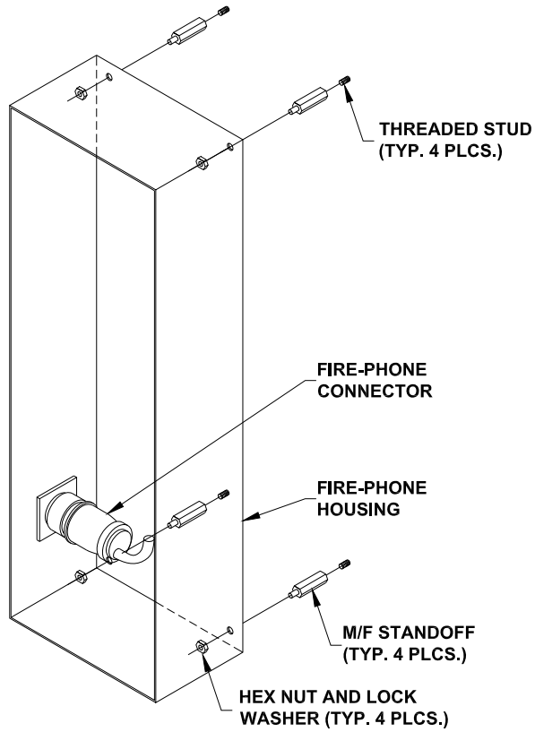
Exhibit 3: Housing Installation
