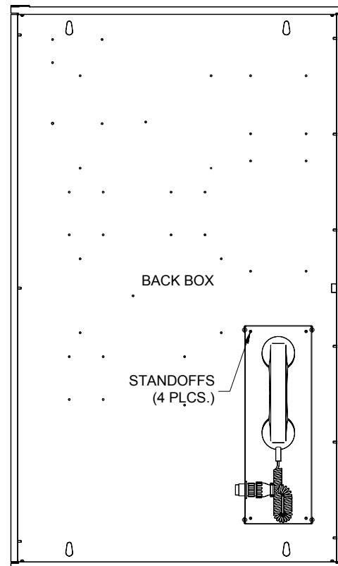
Exhibit 2: Mounting Location - FCC Enclosure
