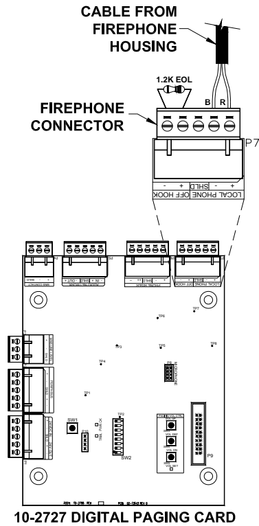
Exhibit 4: Fire-phone Connection to Digital Paging Card
