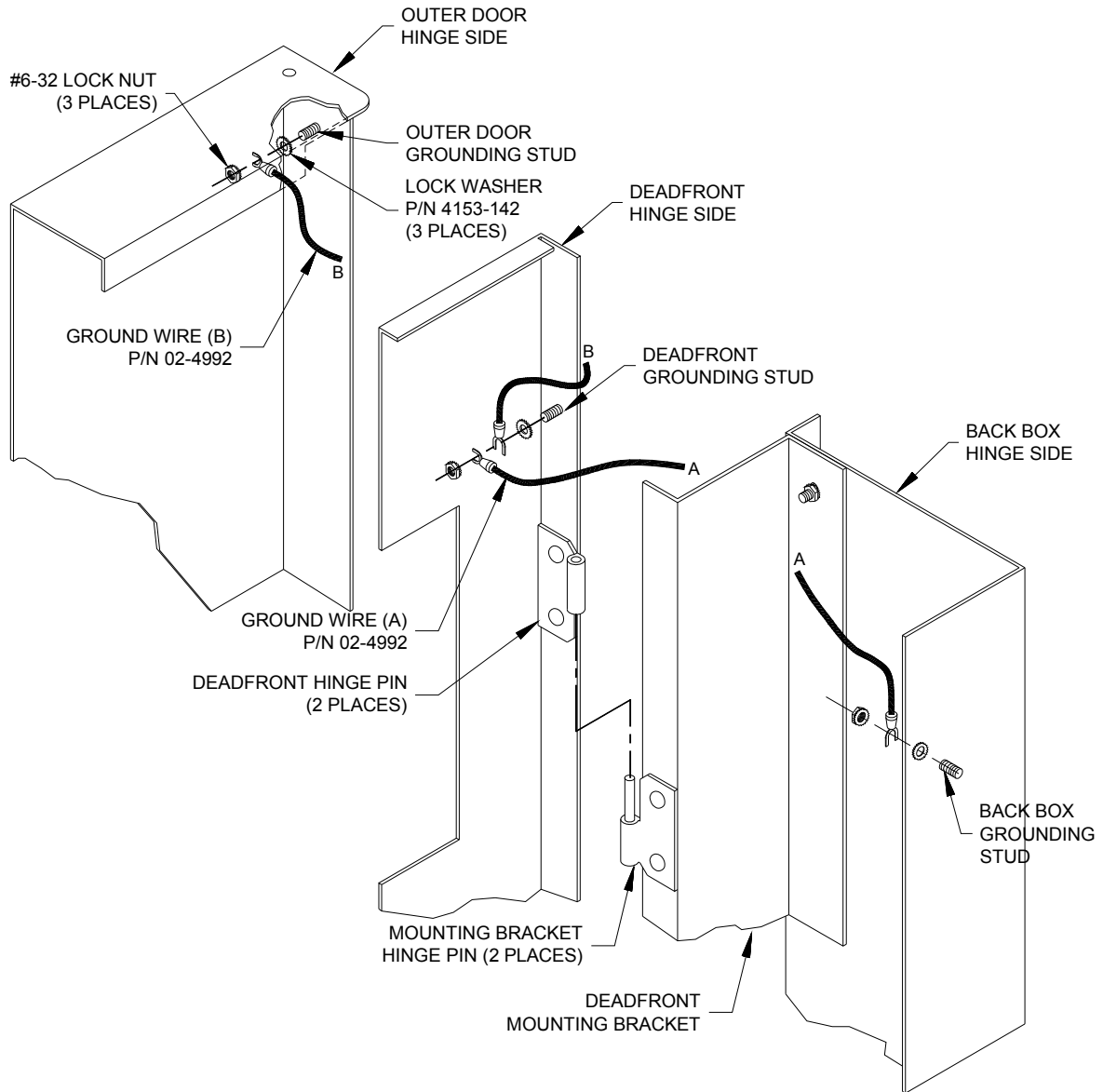
Exhibit 4: Ground Wire Installation
