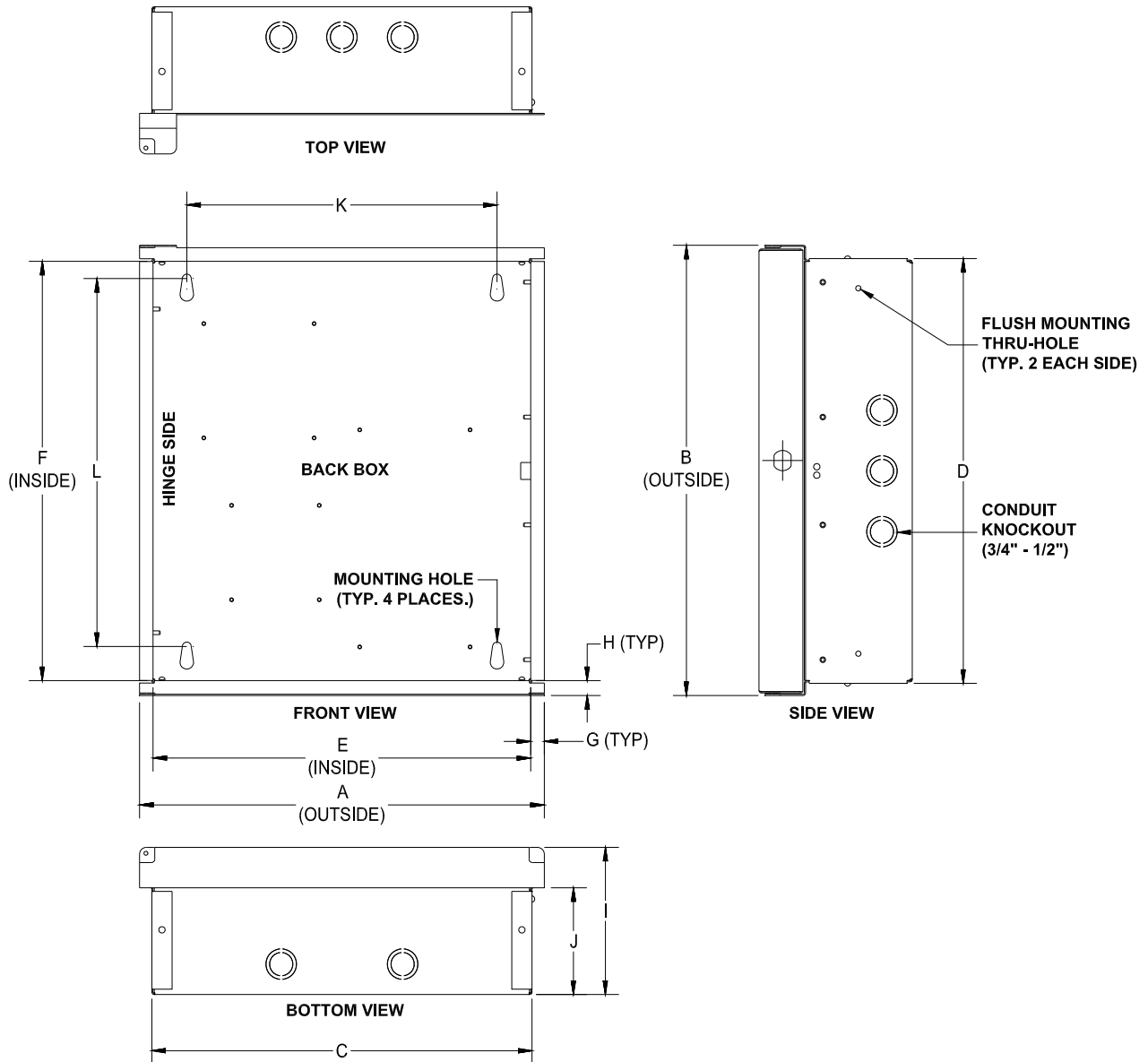
Exhibit 3: Enclosure Dimensions
