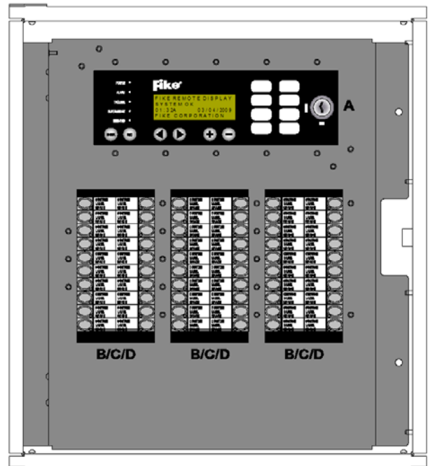
Exhibit 2: Enclosure Layout (shown with dead-front door closed)
