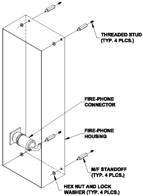
Fire-Phone Housing Installation
