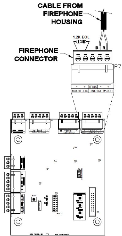
Fire-Phone Connection to Digital Paging Card
