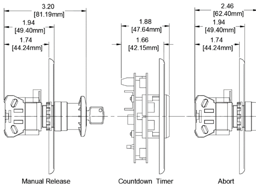
Switch Side View
