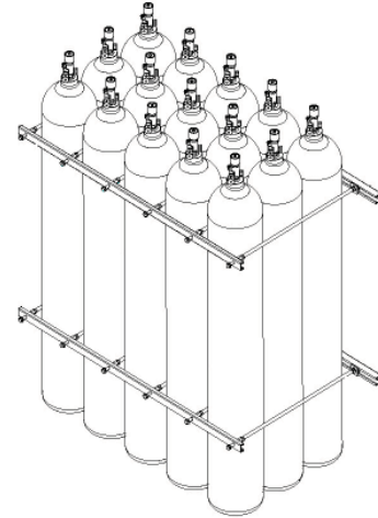
15 Cylinder, Triple Row Racking Assembly
